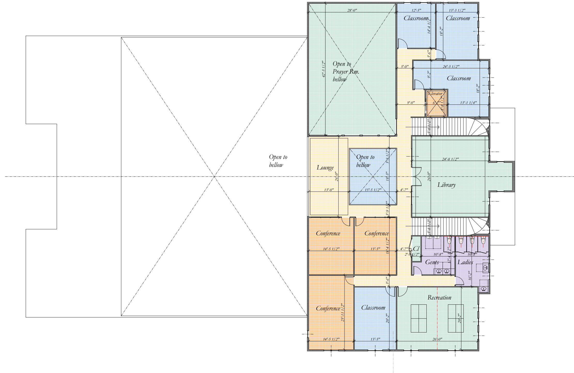
2 nd. Floor plan 6,500 sq.ft.
